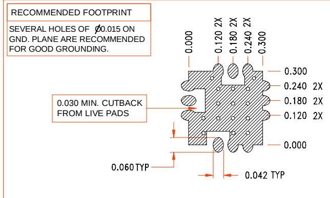
Footprint
