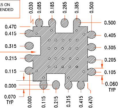
Footprint
