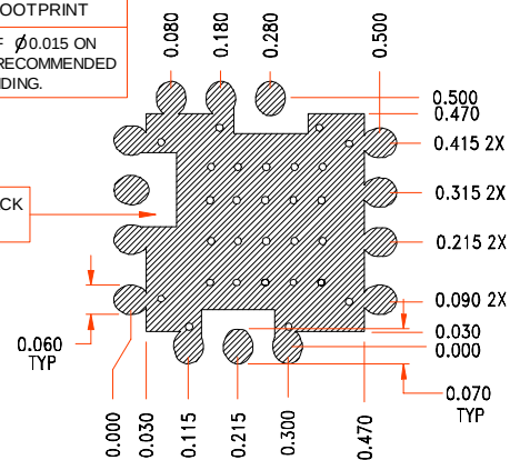
Footprint
